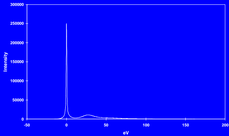
EELS Zero Loss
