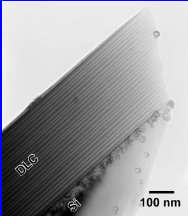
EELS Zero Loss
