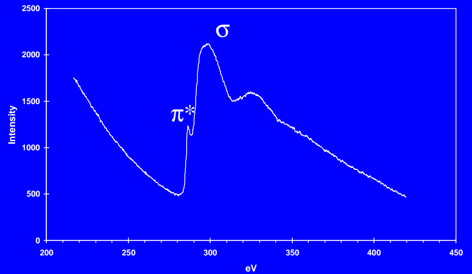
EELS Carbon K Edge (light band)
